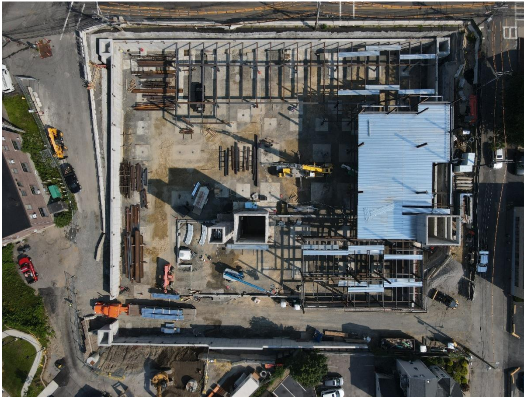
Caption: Aerial photo of construction site on July 27, 2021, by drone to show the layout of the steel beams installed so far, and the metal decking shown to the right.
