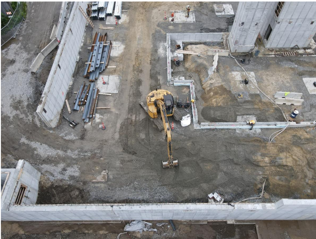
Caption: Aerial photo of construction site take on July 13, 2021. Activities onsite include overall site consolidation, clean-up and preparation for steel installation as shown by the excavator in this photo.
